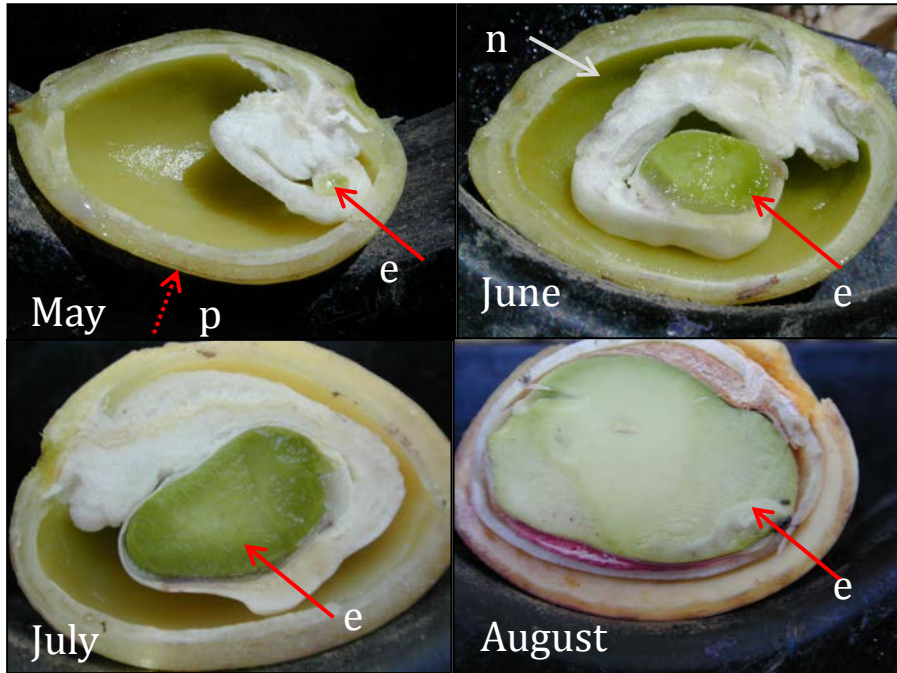
Figure 1. Embryo (e) development does not begin until the pericarp (p) has reached its maximum size. Although endocarp (n) hardening is initiated prior to embryo development, these two processes do occur simultaneously (Allen et al., 2014).
