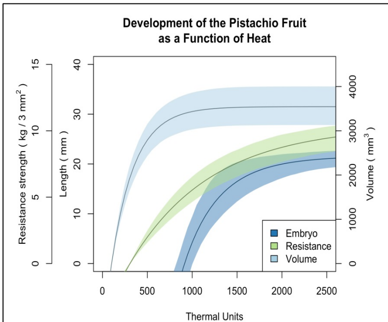
Figure 2: Summary of the three growth stages of a pistachio fruit using a non-linear model. The data are a summary of five cultivars, at six sites over two seasons. The growth curves for the stage 1 pericarp growth (volume), light blue curve, was generated using data from length, width, and height data from 2013 and 2014 and applying it to the equation for the volume of an ellipsoid. The curve for stage 2 (penetrometer), green curve, was derived from the recorded hardness of lbs/ 3mm 2 over the 2013 and 2014 growing seasons. Stage 3, kernel growth, (embryo length), dark blue curve, was measured from detectible embryo presence through harvest for the 2013 and 2014 growing seasons. The shaded region shows the 95% credible interval.
